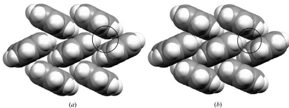
Figure 6 Space-filling plots for naphthalene at (a) ambient pressure and (b) 2.1 GPa. Examples of reduction in structural voids are shown in the circled area.
