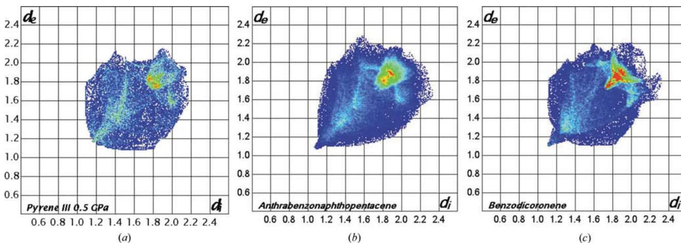
Figure 14 Fingerprint plots for (a) pyrene-(III) at 0.5 GPa, (b) anthrabenzenaphthopentacene (CSD reference code BOXGAW01) and (c) benzodicyronene (CSD reference code YOFCUR).
