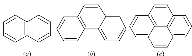
Figure 1 Molecular structure of (a) naphthalene, (b) phenanthrene and (c) pyrene.
